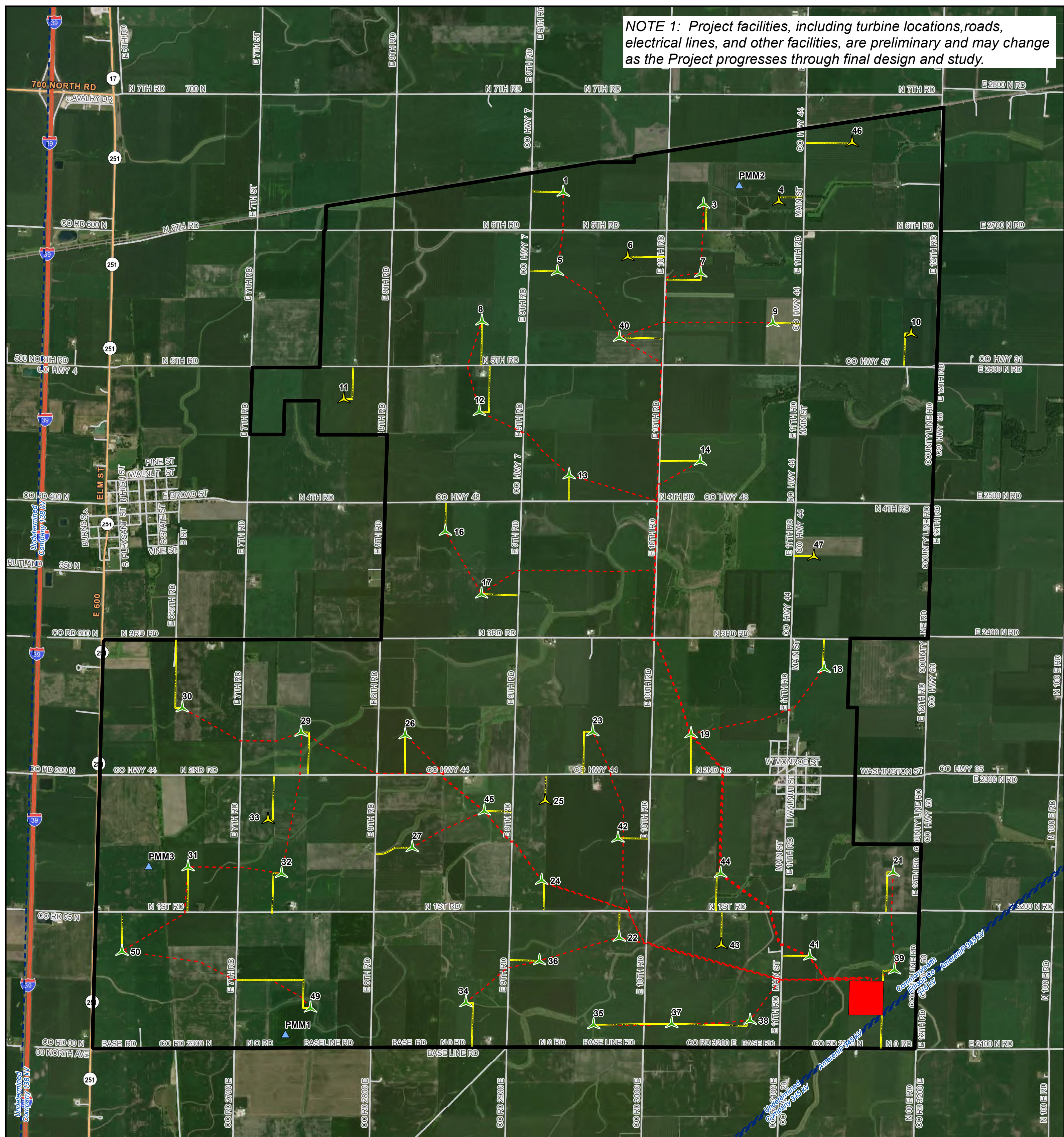
Figure 3 Preliminary Project Layout Osagrove Flats Wind Project
